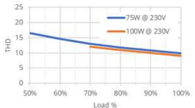
Total Harmonic Distortion vs Load
